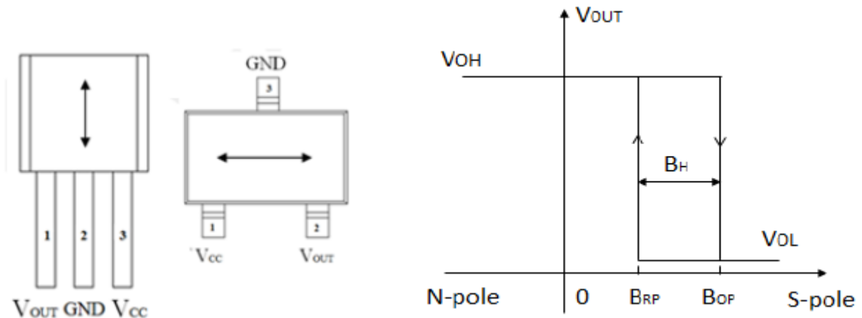
Sensing direction of magnetic field
