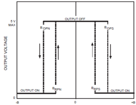
Magnetic Flux
