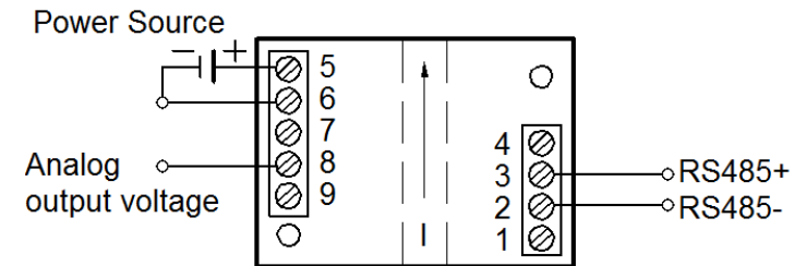
Fig.3 Pin Definition
