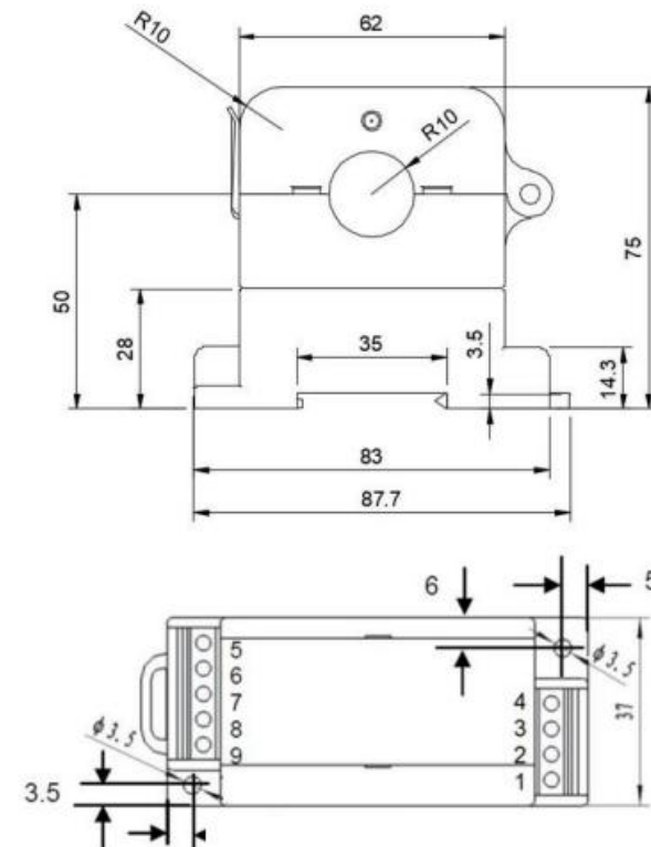
Fig.2 Case Dimensions
